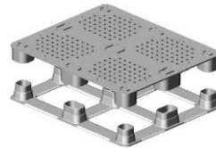
Isometric Exploded Illustration of Structural Foam Pallet
